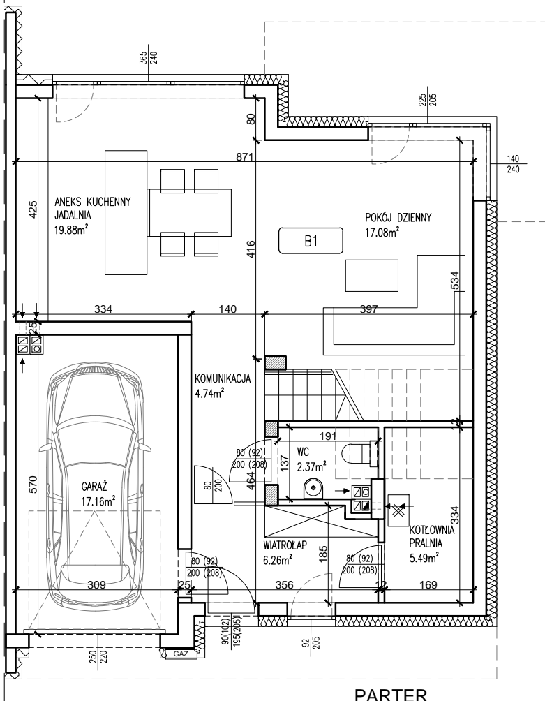
PARTER
